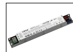
Driver LIFUD dimmable DALI2 \overline{PUSH} 37W max. 75-400mA (SUR COMMANDE)
