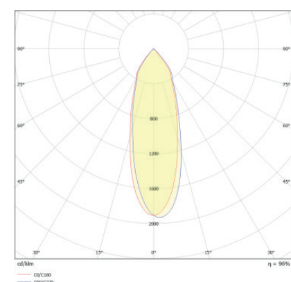
825002 Driver LIFUD dimmable DALI2 PUSH 20W (réglage 300mA)
