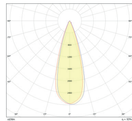
825002 Driver LIFUD dimmable DALI2 PUSH 20W (réglage 500mA)
