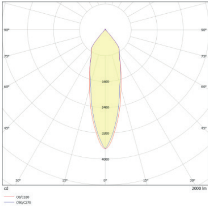
825002 Driver LIFUD dimmable DALI2 PUSH 20W (réglage 500mA)
